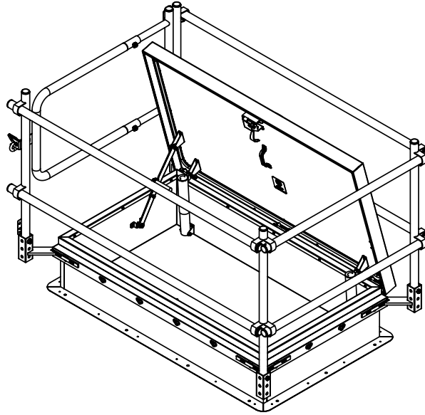
SAF-T HATCH™ WITH GATE EXIT ON WIDTH Typical for Stair Access Hatches
