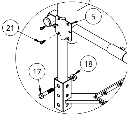
DETAIL D SCALE 1 : 8
