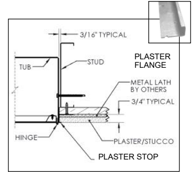
TRIMLESS RECESSED FLANGE FOR 3/4" PLASTER (P)
