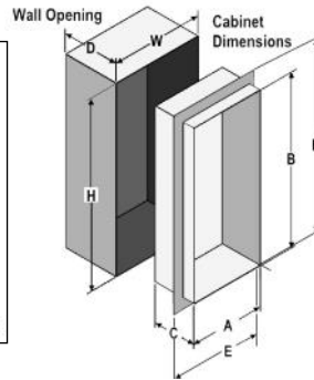
TRIMLESS RECESSED FLANGE FOR 3/4" PLASTER (P)
