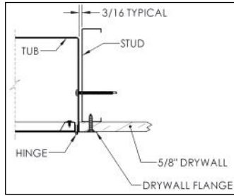
TRIMLESS FLANGE FOR 5/8" DRYWALL (W)
